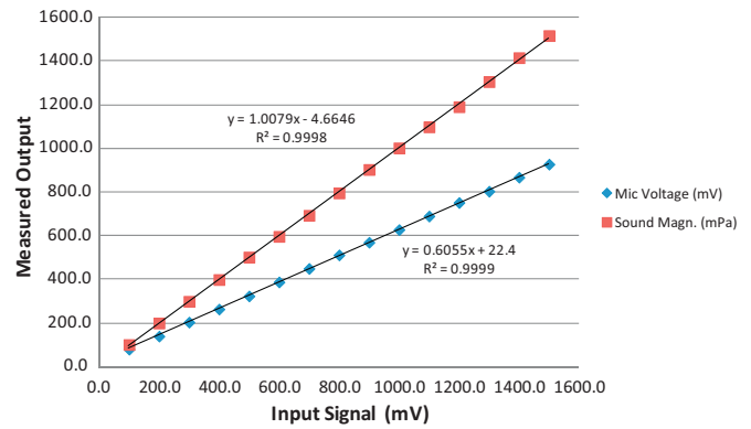
Fig. 1. Results from the amplified microphone gain calibration test at 1000 Hz. Test compared input signal (mV) to microphone output (mV) as well as the SPL response from an NIST traceable sound meter (dB) which was converted from SPL (dB) to pressure (mPa).
