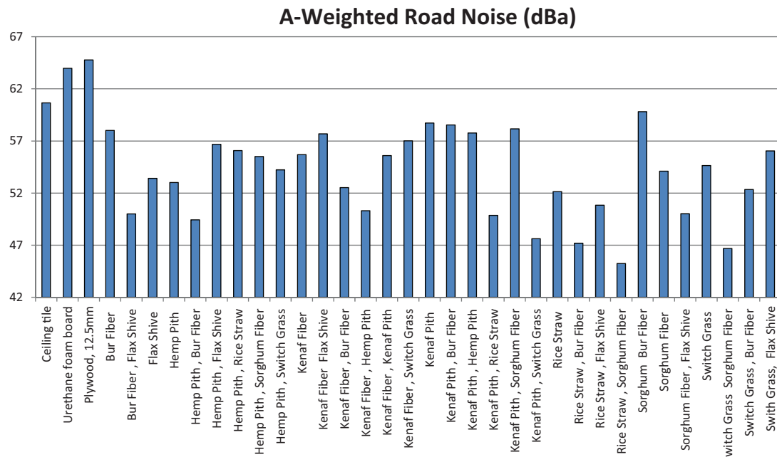
Fig. 4. Results of the entire group of composite mixtures that were tested. Results shown are the acoustic performance for perceptual response of road noise for each of the tested composite mixtures (integrated A-weighted response with typical road noise excitation).
