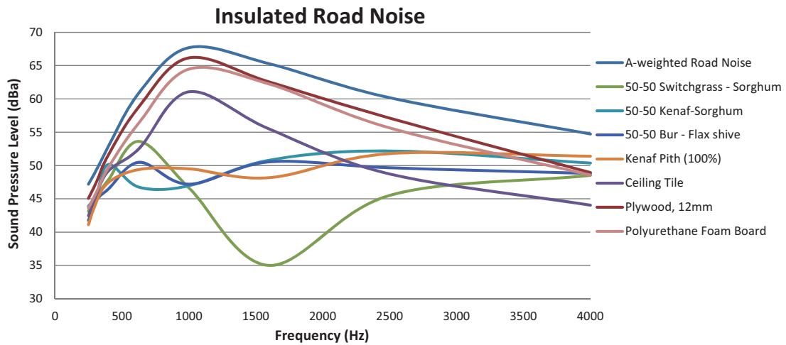
Fig. 3. Test comparing the audio spectrum, A-weighted with typical road noise excitation, between mycelium based acoustic absorption boards ranging from best to worst performers alongside a few traditional absorbers for reference, such as plywood and a typical 25 mm thick poly-urethane insulation board.
