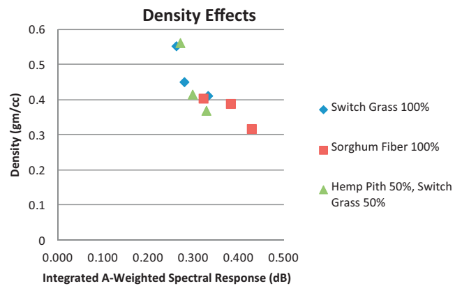
Fig. 5. An inverse relation to density was observed between replications on a per case basis. There was not however a significant impact of density on a global basis.
