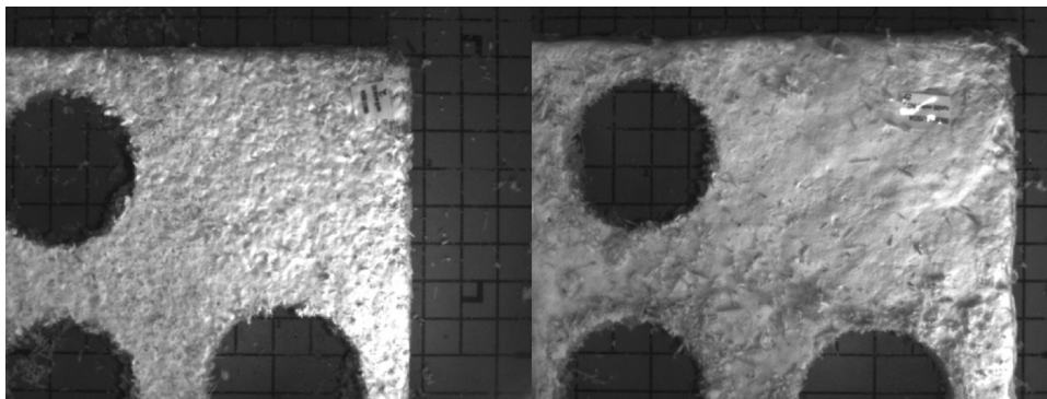
Fig. 6. Comparison images of the varying surface texture that occurred when mycelium was grown on various substrates. On the left is a picture of 50% kenaf pith and 50% cotton bur fiber that produced a nice compact dense board, but a rough surface texture. On the right is a picture for 50% kenaf pith and switch grass that yielded a smoother surface texture.
