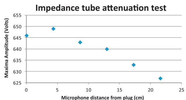
Fig. 2. Test examining the attenuation at maxima locations as a function of microphone distance from hard brass reflector, providing a near perfect reflection at 1600 Hz.
